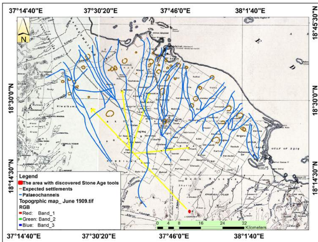
Fig. 15 The topographic setting of the study area includes the Agig and Tokar (the study area with the discovered potential settlements and paleoriver) regions
